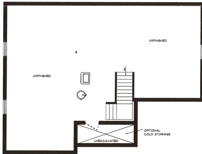
FOUNDATION PLAN
